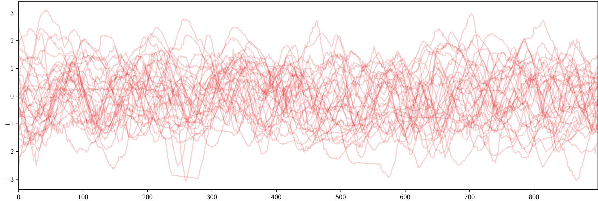
WormsTwoClass Class 1
